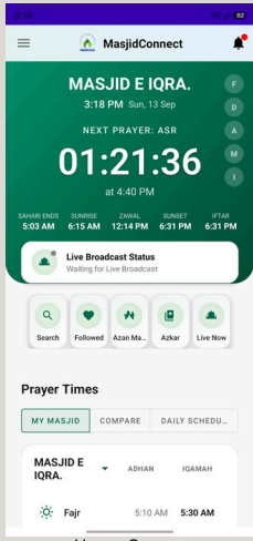
Home Screen
